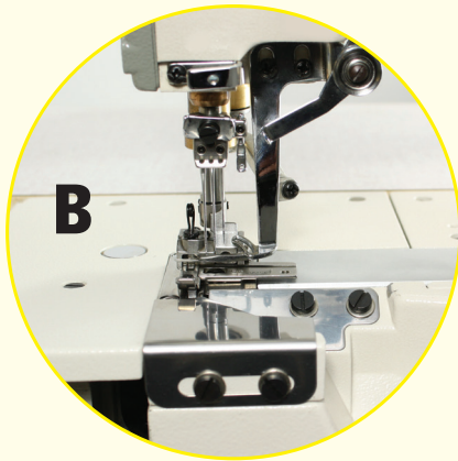
FB 3603-64 BFC-DD BINDING OPERATION
