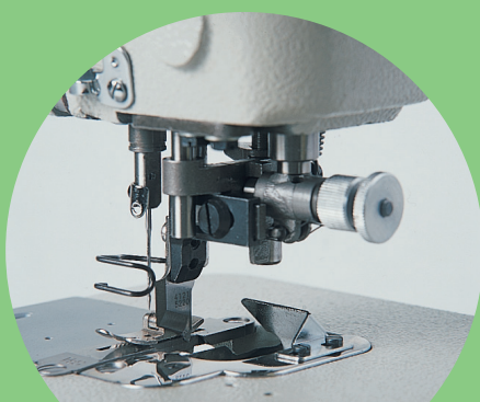
SIDE KNIFE ATTACHMENT
